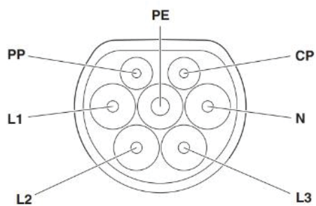
Charger plug
