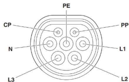
Vehicle connector
