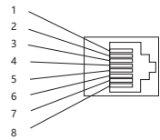
RJ45 female connector
